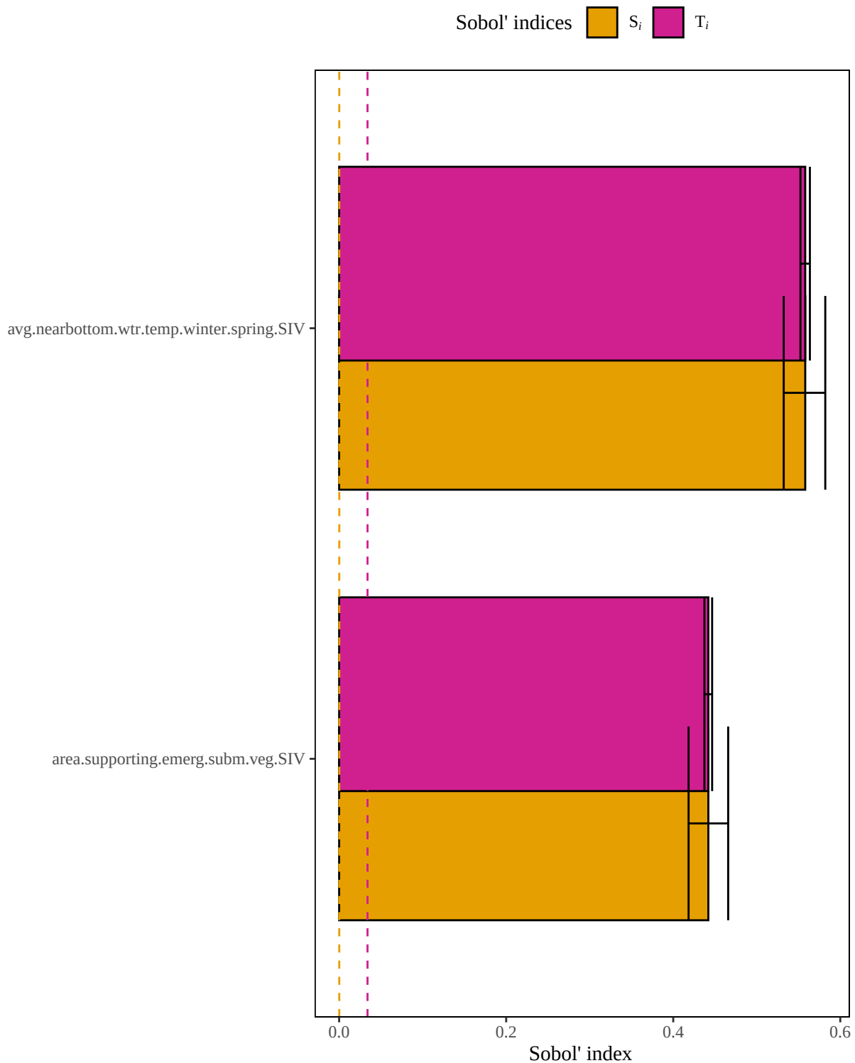
Figure 4. Results of a sensitivity analysis for the americanshadEstu model based on an arithmetic mean structure. Dashed lines represent baseline numerical approximation error for S_i and T_i ( i.e. , dummy variables).
