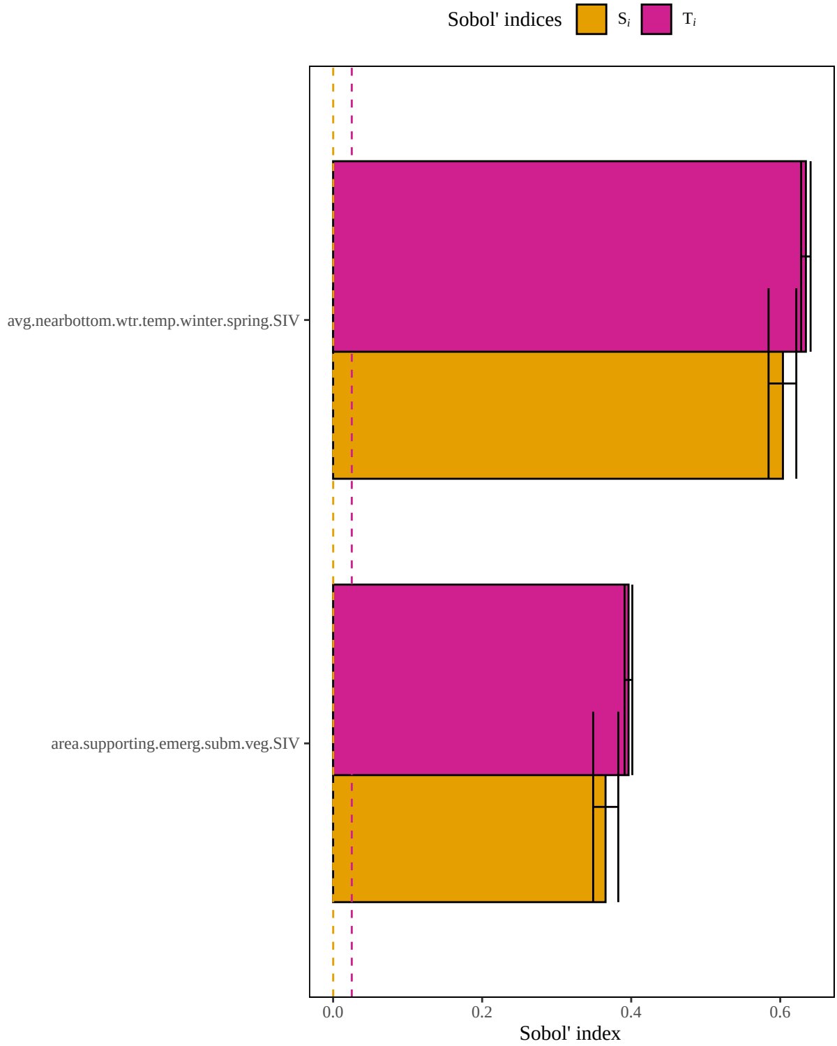
Figure 5. Results of a sensitivity analysis for the americanshadEstu model based on a geometric mean structure. Dashed lines represent baseline numerical approximation error for S_i and T_i ( i.e. , dummy variables).
